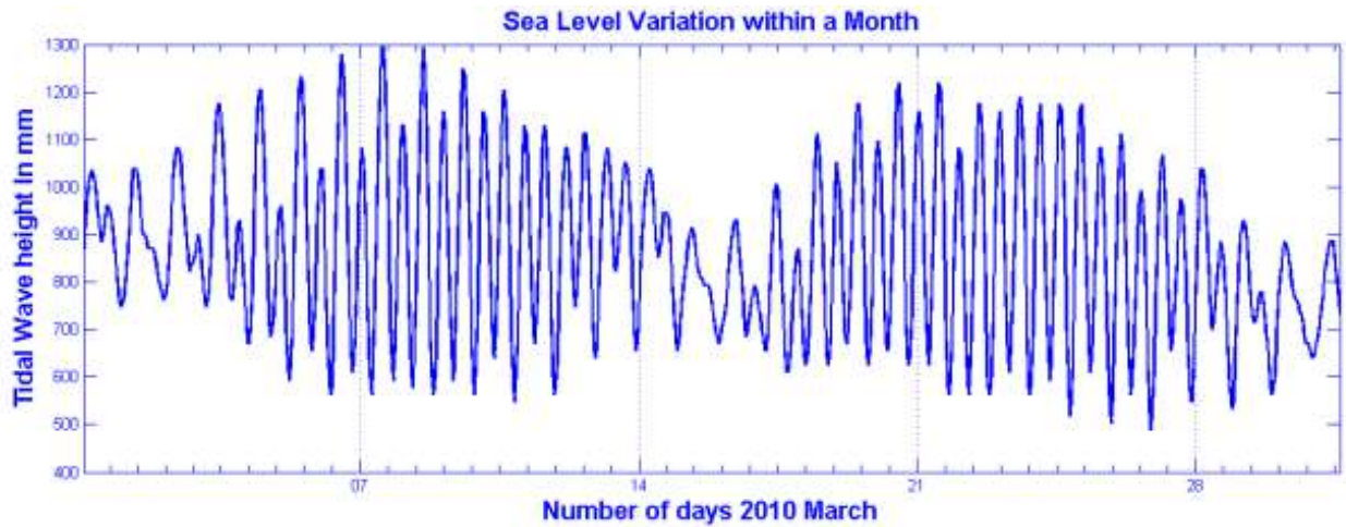
Figure 3. Monthly mean sea level variation in the west coast of Sri Lanka
