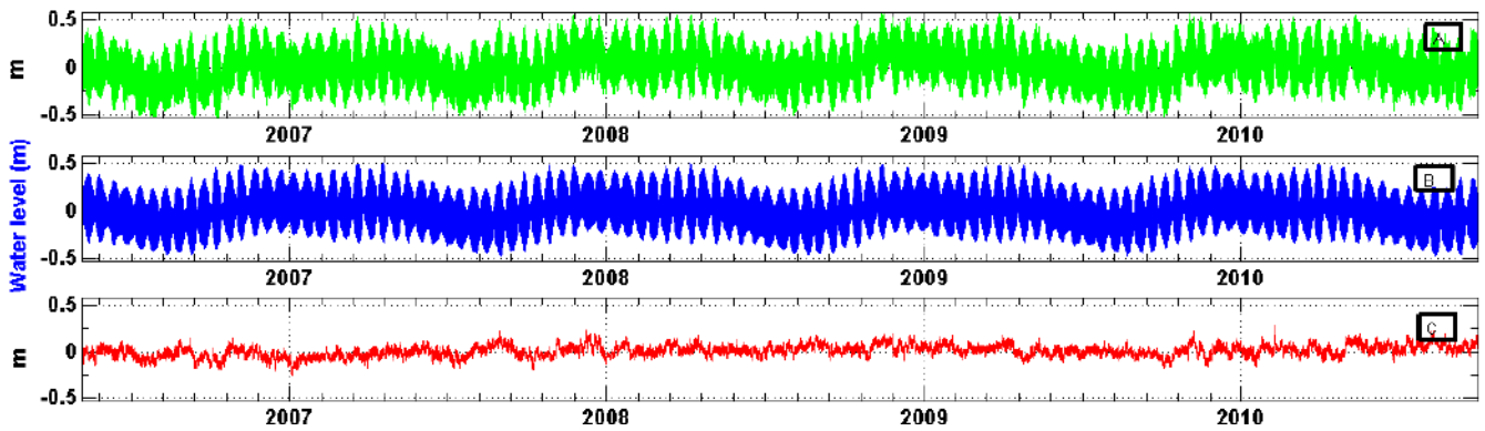
(a). The green line shows the actual tide gauge one minute frequency reading (b). Blue line shows the predicted tidal variation (c). red line shows residual sea level variation
